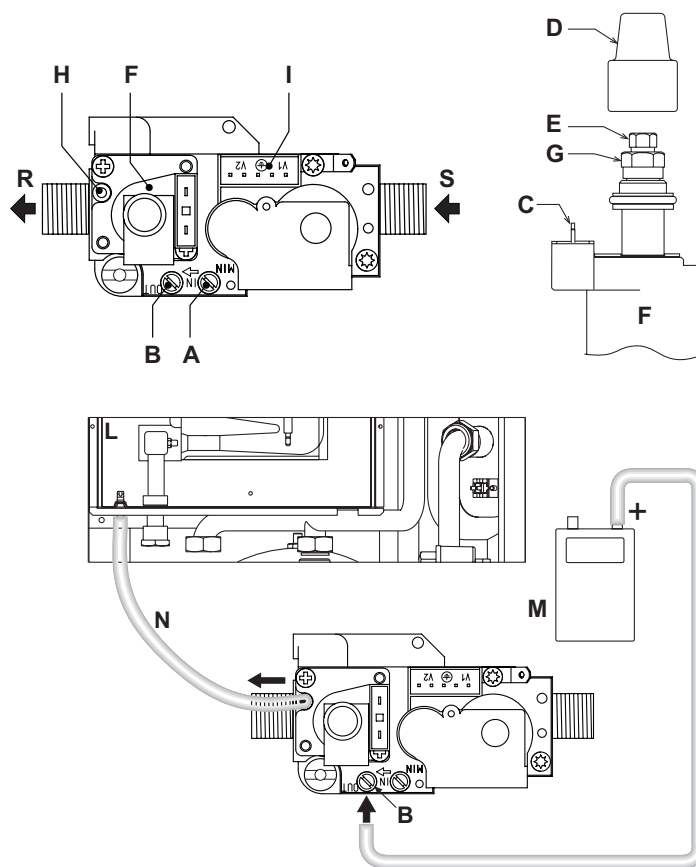
fig. 29 - Valvola gas
